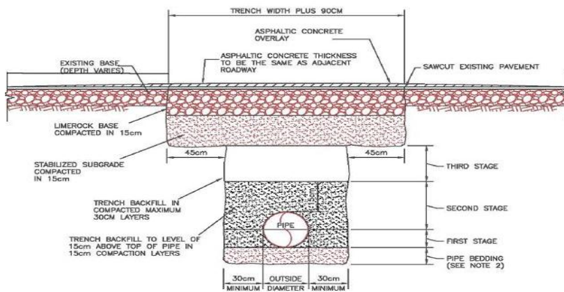
Trench restoration Installation details
