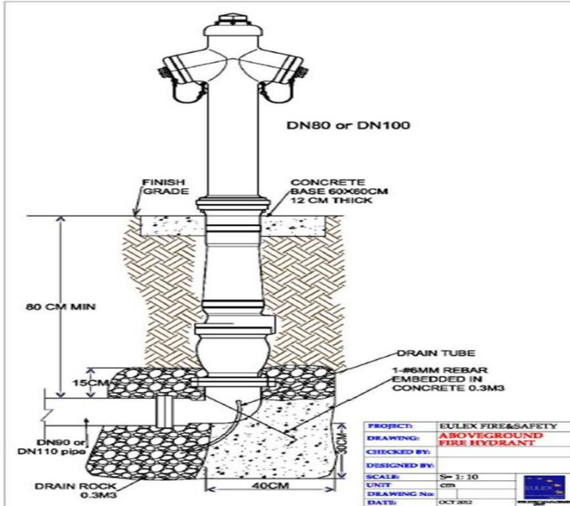
Above ground Fire Hydrant Installation details
