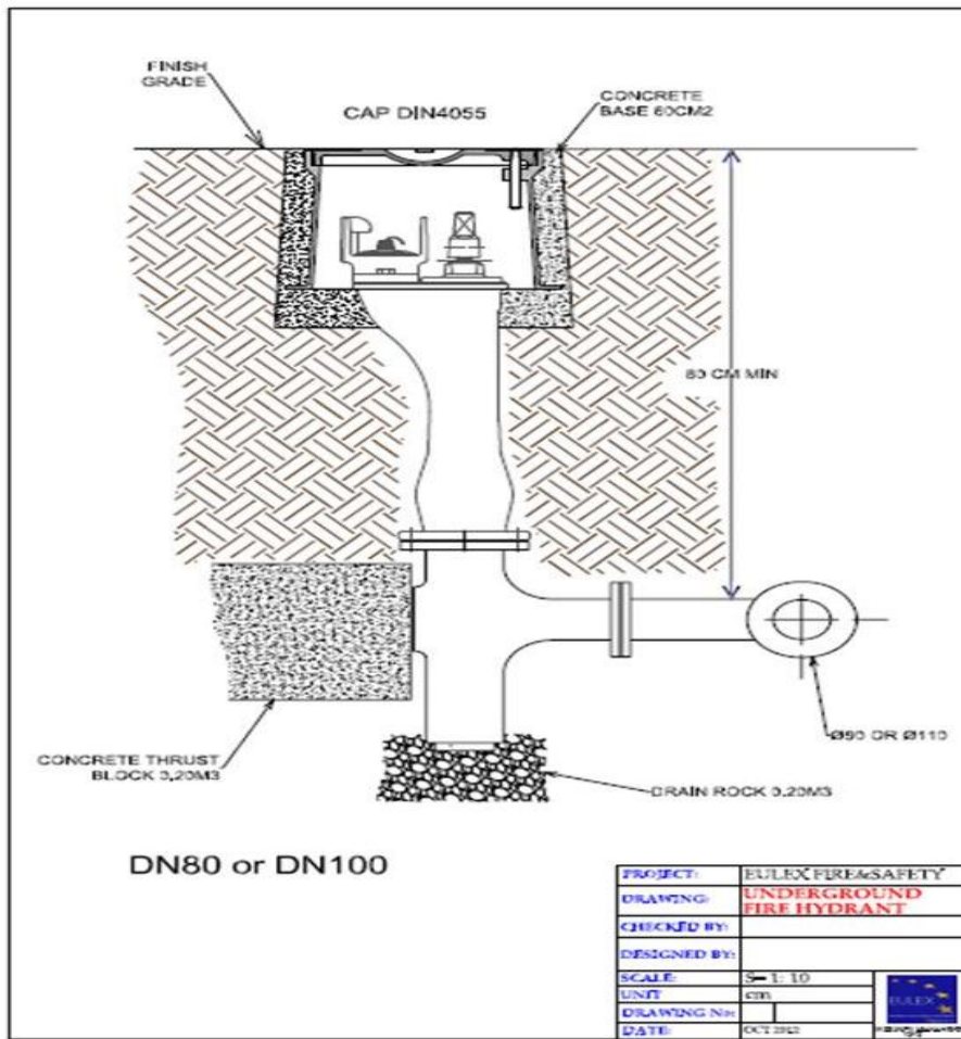
Underground Fire Hydrant Installation details
